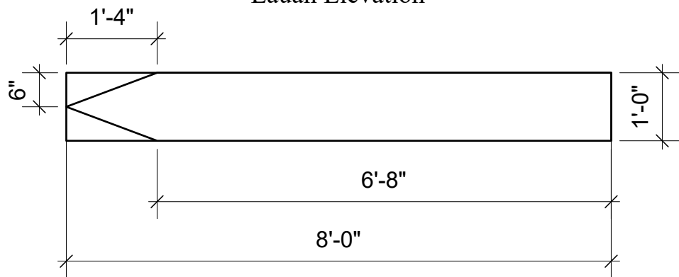
Lauan Elevation
