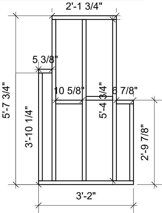
Ground Plan
