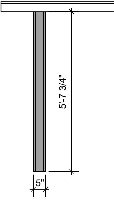
Side Elevation
