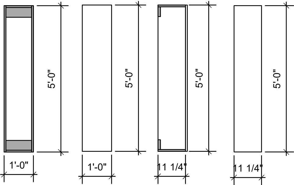
Side Elevations
