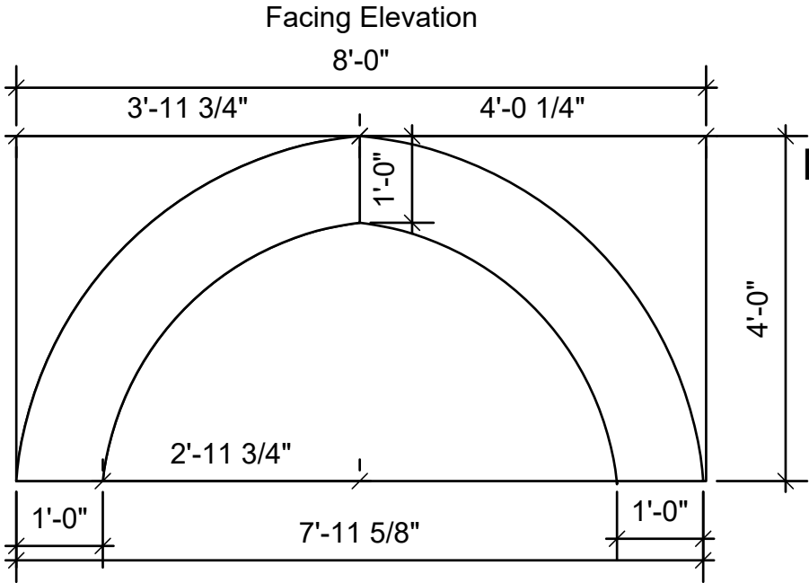
Front Elevations
