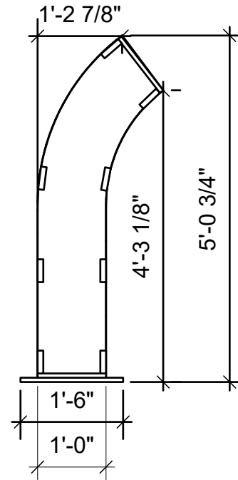
Rib 2 Side Elevation
