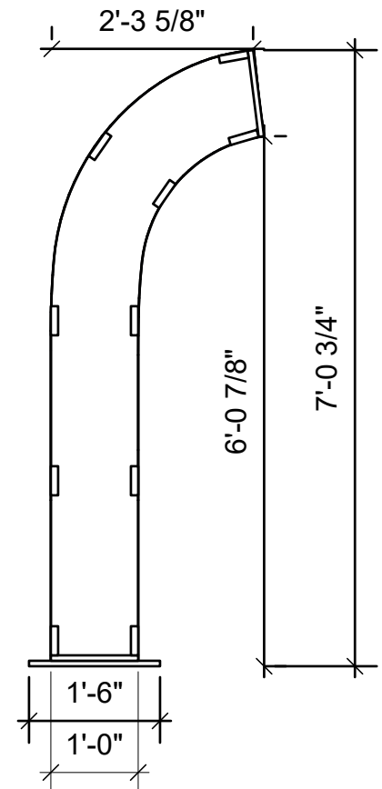
Rib 3 Side Elevation
