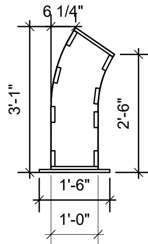
Rib 1 Side Elevation
