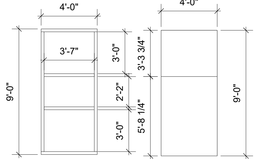
Lauan Layout
