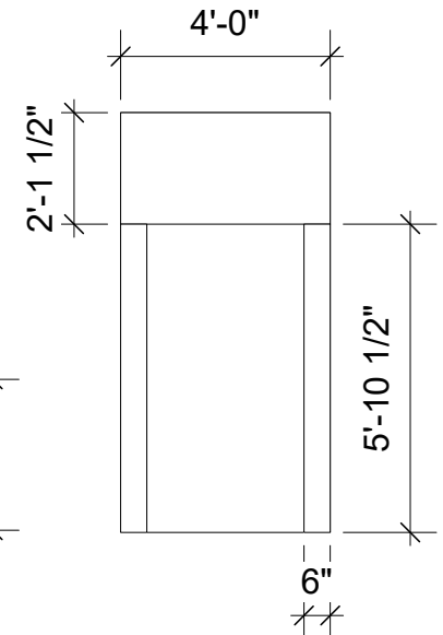
Lauan Layout
