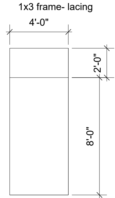
Lauan Layout
