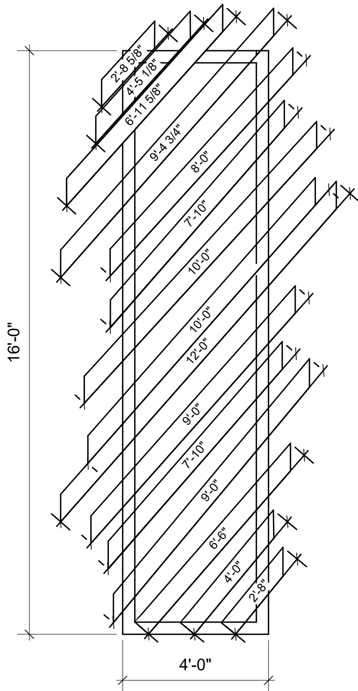
Front Elevation
