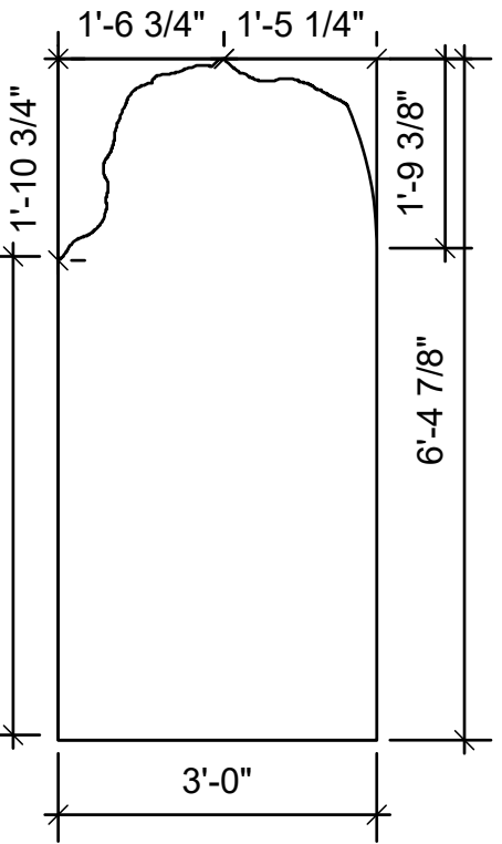
Door 2 Facing Elevation
